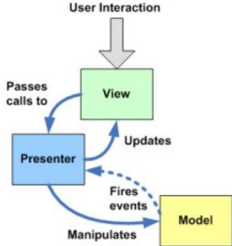
Model-View-Presenter
