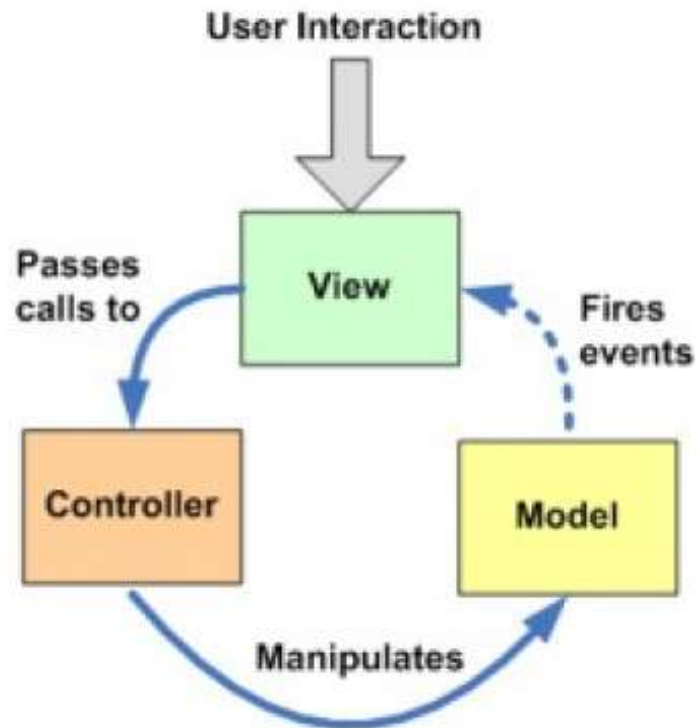
Model-View-Controller
